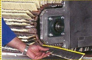
The sanding belt consists of easy interchangeable brush segments
